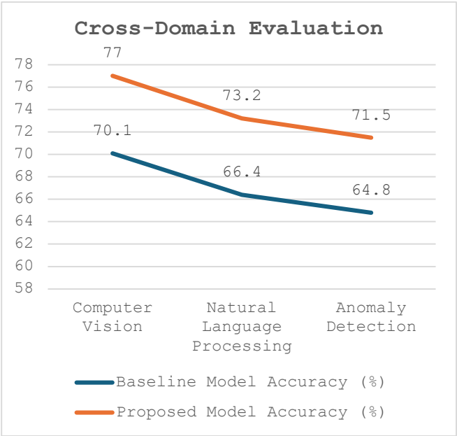
FIG: Cross-Domain Evaluation
